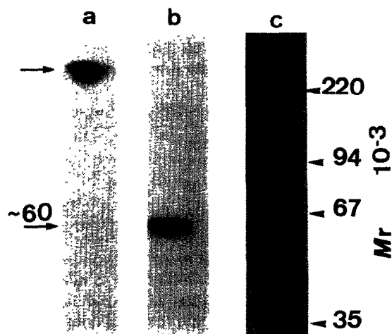
Fig. 4. Autoradiographs of SDS linear 10–16% (w/v) acrylamide gel separation of partially purified asparaginase. Lanes: (a) phosphorylated by [\gamma\text{-}^{32}\text{P}]\text{ATP-Mg}^{2+} , (b) ^{32}\text{P} phosphorylated and then dephosphorylated by calf-intestinal alkaline phosphatase, (c) dephosphorylated and then ^{32}\text{P} phosphorylated. The general conditions of these assays are described in sections 2.3 and 2.4. M_r values have been determined using markers in parallel.
