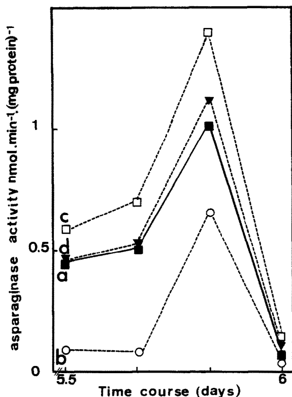
Fig. 3. Freezing and phosphate effects on the time course of asparaginase activity: 50 mM Tris ( \text{Cl}^- , pH 8.6) enzyme solutions were frozen at -20^\circ\text{C} for 1 week then thawed and incubated at 4^\circ\text{C} for 1 h before asparaginase assay. Control before (a) and after freezing (b). Thawed enzyme solutions preincubated in the presence of \text{ATP-Mg}^{2+} (c) or 66 mM \text{P}_i (d). Experiments were performed 3 times with similar results.
